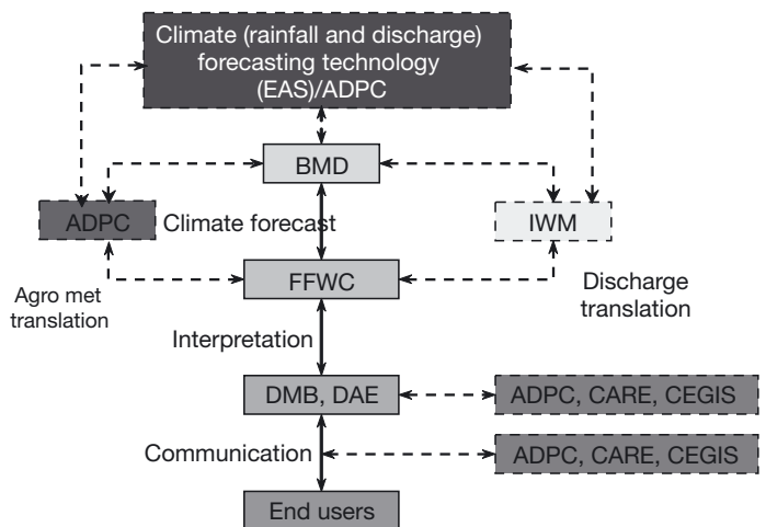
Fig. 1. Linkages established between different partnering institutions for long lead (1 to 10 d) forecast of rainfall. Solid lines denote flow of forecasts and products while broken lines indicate coordination between the institutions involved, namely Asian Disaster Preparedness Centre (ADPC); GeorgiaTech – Earth Atmospheric Sciences (EAS); University of Colorado, which collaborated with EAS; Bangladesh Meteorological Department (BMD); Flood Forecasting and Warning Centre (FFWC) of the Bangladesh Water Development Board (BWDB); Disaster Management Bureau (DMB); Department of Agricultural Extension (DAE); Center for Environmental and Geographic Information Services (CEGIS); and CARE Bangladesh
